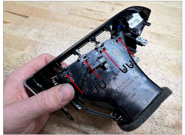
1b Then release 4 clips on the underside of the vent
