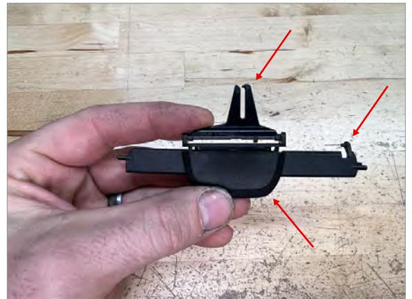
4 Install the slider onto the bottom slat as shown (Note the position of the fork, slider, and slat)
