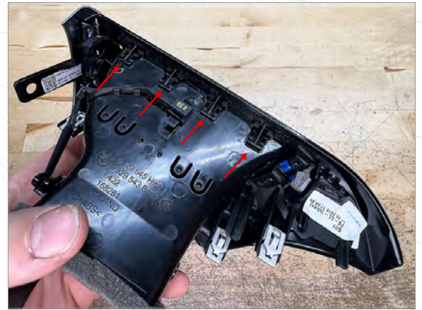
9b Snap 4 clips on bottom into place
