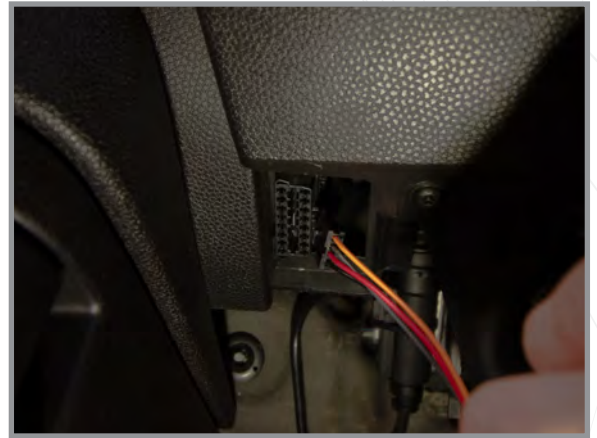
8a Feed the small end of the OBD2 cable up through the hole next to the OBD2 port and out the side of the dash. Reconnect main harness.
